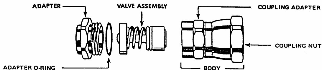
Figure 7 Aeroquip Female Coupling Parts
